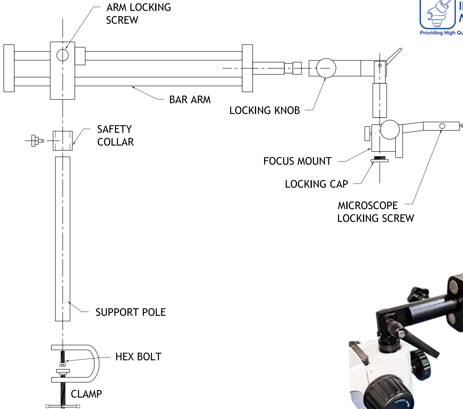
BALL BEARING ARM ASSEMBLY DIAGRAM
